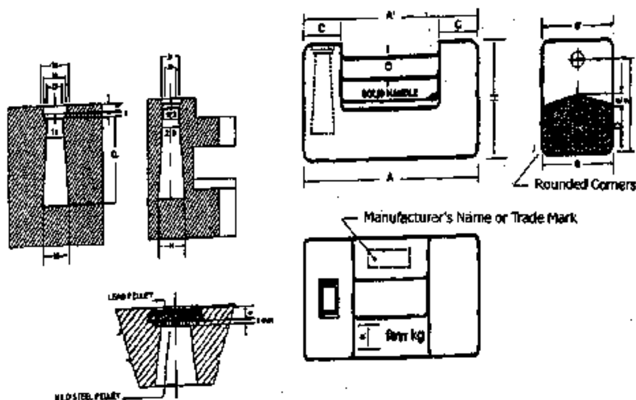
Paralleliped Weight Type 2
