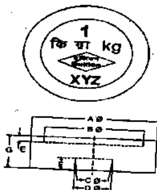
Flat Cylindrical Bullion Weights Figure - 7
