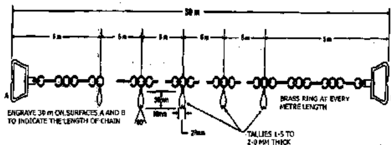
30-METRE CHAIN FIGURE-28
